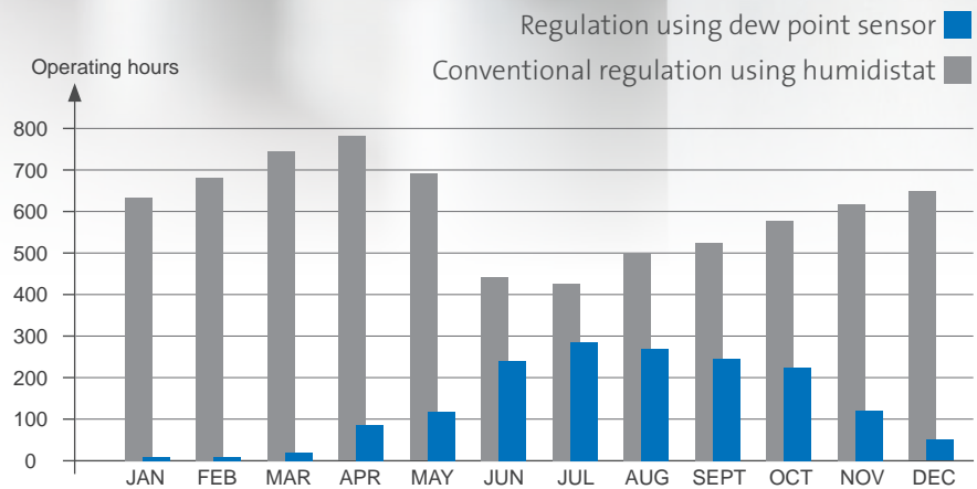
Exemplary reduction of operating hours through needs-optimized regulation in a waterworks
